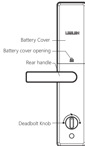
Rear Panel
